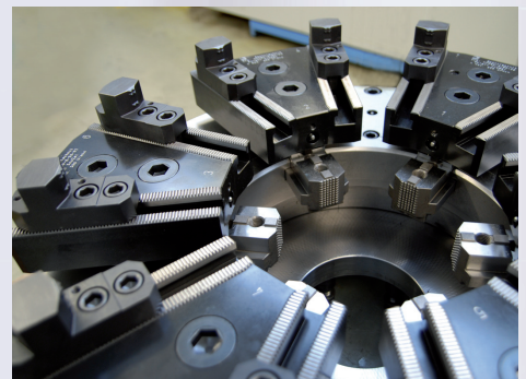
Variable positioning of the clamping jaws on the pedulum segments
